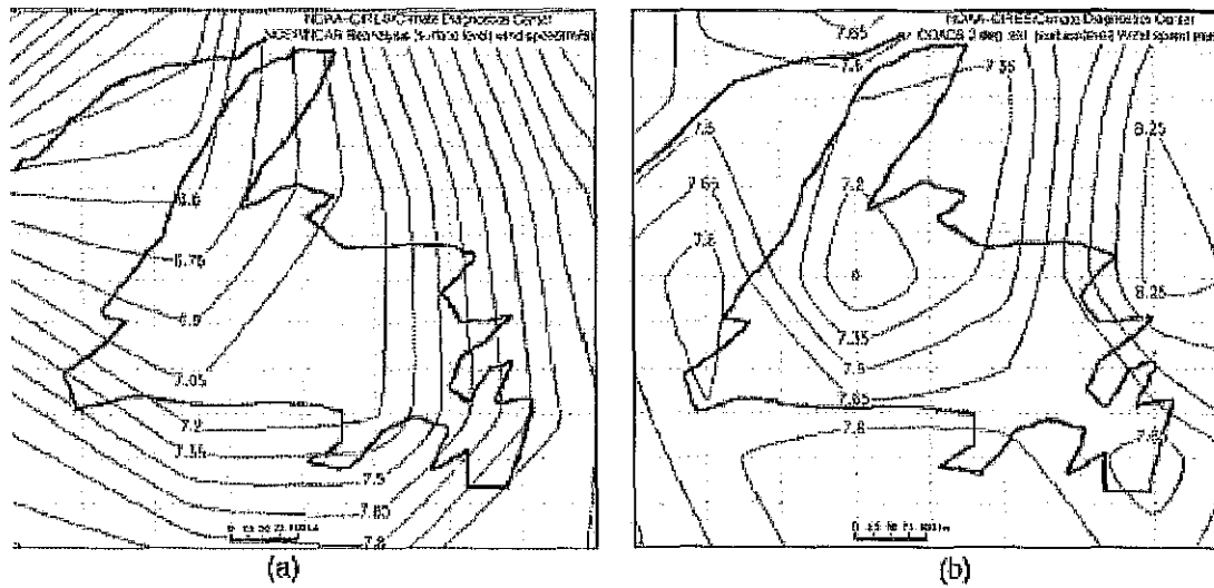
Fig. 5. Wind map of Newfoundland at surface level (m/s) (a) CDC derived NCEP Reanalysis Product averaged over Jan 1948-Aug 2003 (b) COADS (2 deg. standard) data averaged over Jan 1800-Dec 1997.
